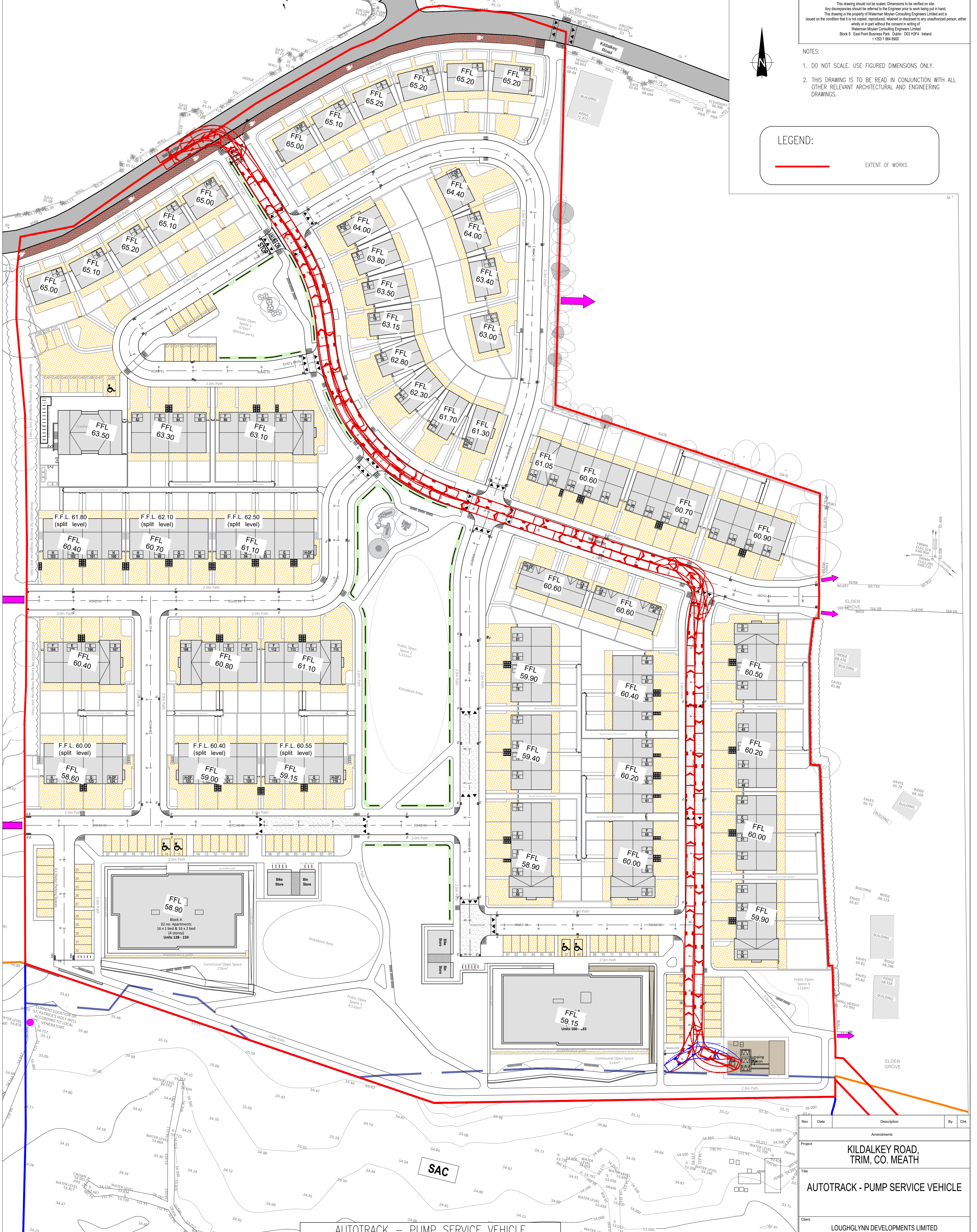
AUTOTRACK - PUMP SERVICE VEHICLE SCALE 1:500 @A1
